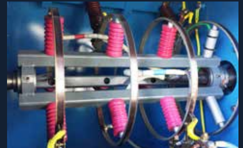
Obsolete HV Collector and Slipping Assembly
