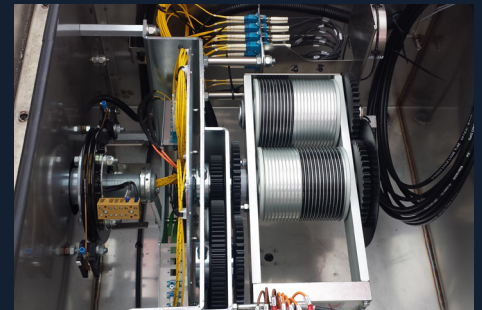
FORA unit after CavotecReman
